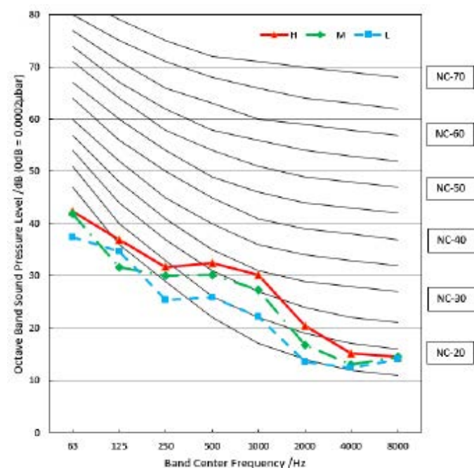
KPD-35 DR13
