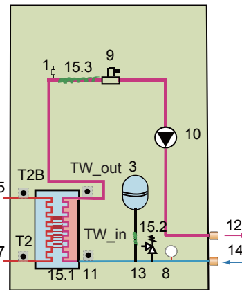
Monofásica, 5/7 kW
