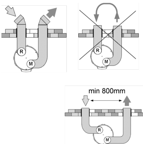
COMPAK KHP 16 190S
