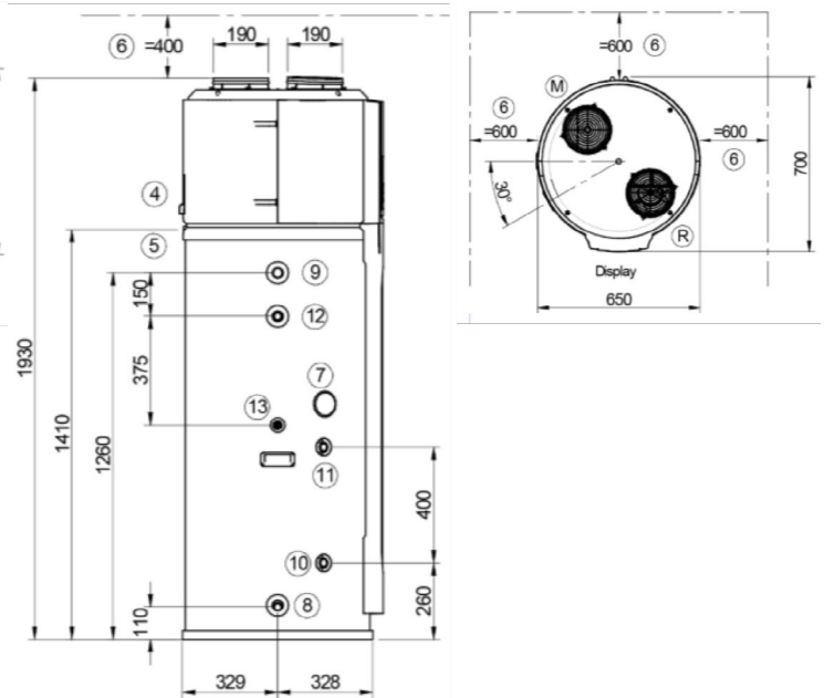
COMPAK KHP 23 300S
